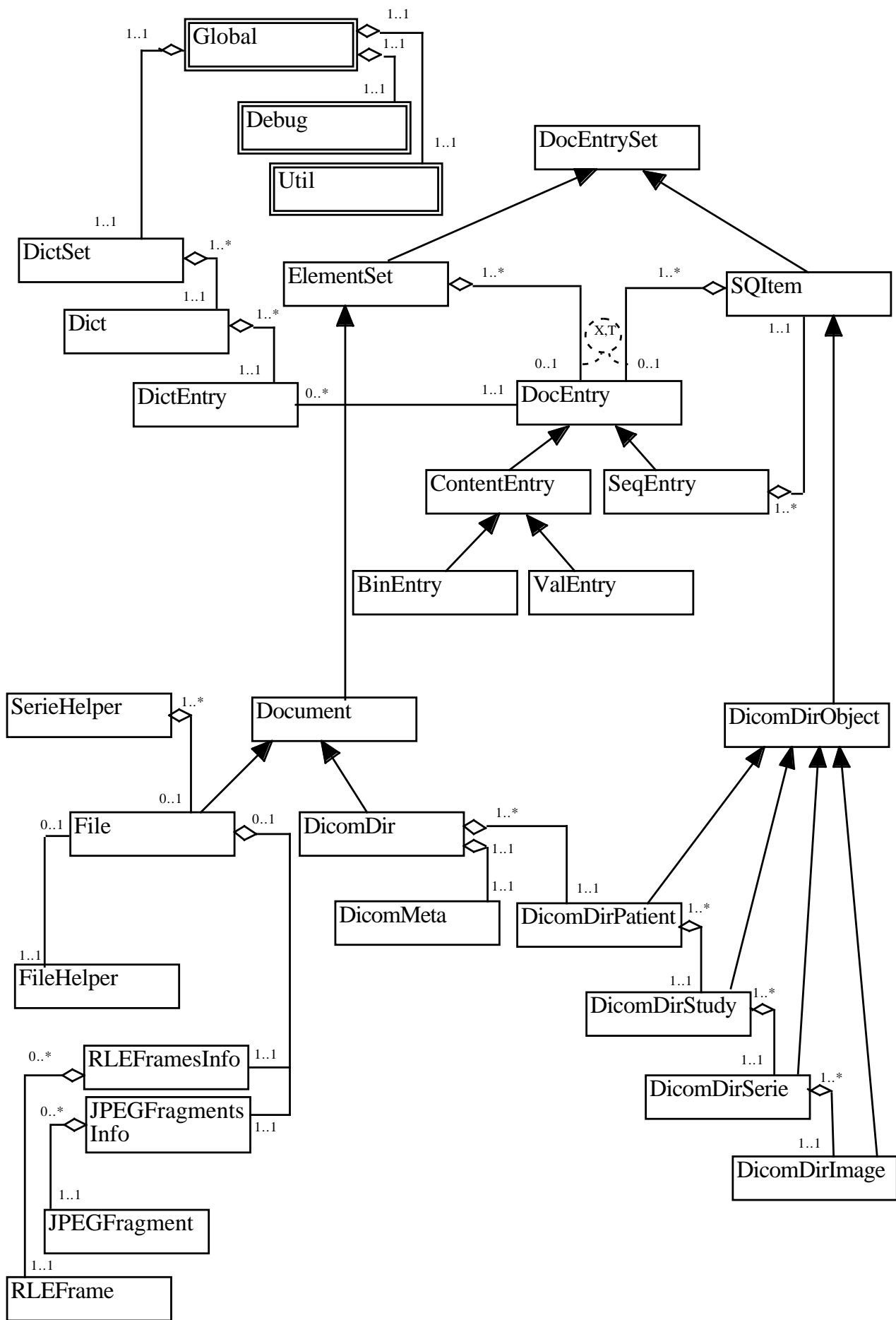
gdcmm UML Classes Diagram
